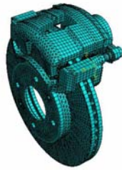
Figure 2: Finite element model of a disc brake assembly
