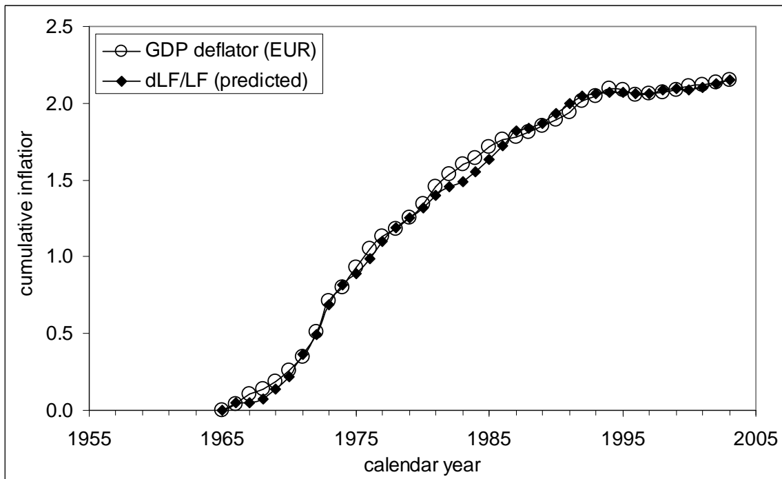
Fig. 10. Comparison of the observed (EUR GDP deflator) and predicted inflation in Austria. The upper frame displays annual readings and the lower one – cumulative inflation since 1965. Notice a major change in labor force definition between 1981 and 1987 (OECD, 2005). The periods before and after 1986 are described separately.
